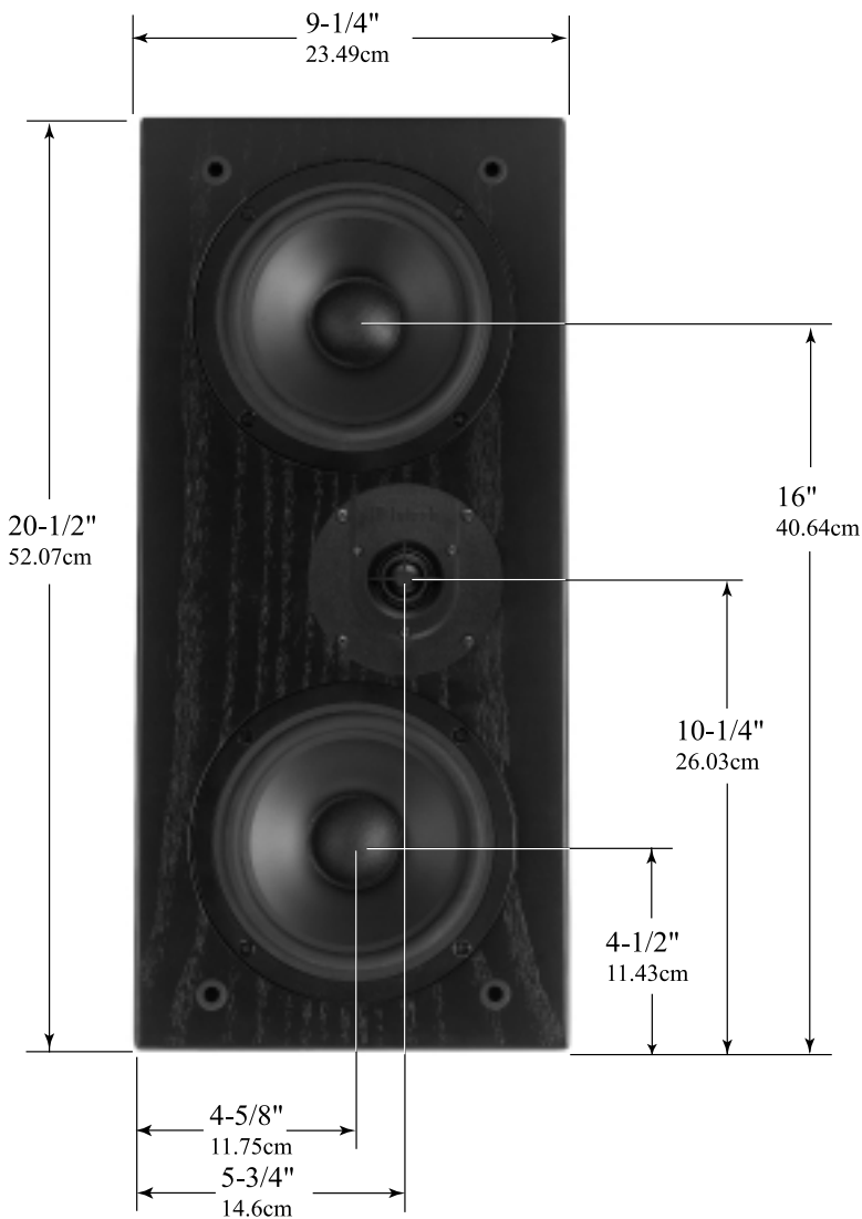
Front View of HT-5 with Grille Removed
