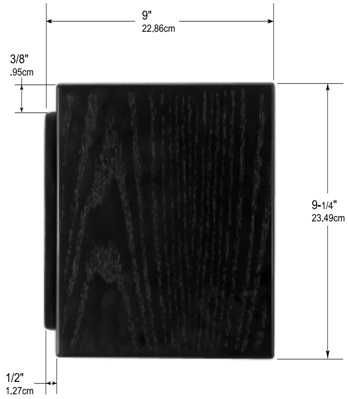
Top View of HT-5 with Grille
